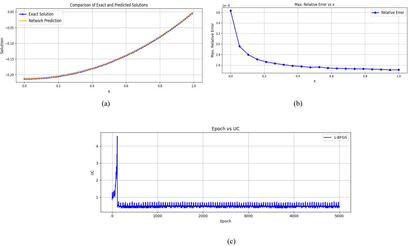
Figure 4. Comparison of predicted and exact solutions for the thermal explosion problem: (a) solution profiles, (b) maximum relative error at different spatial points x , and (c) optimizer update cost versus training epochs demonstrating convergence behavior.
