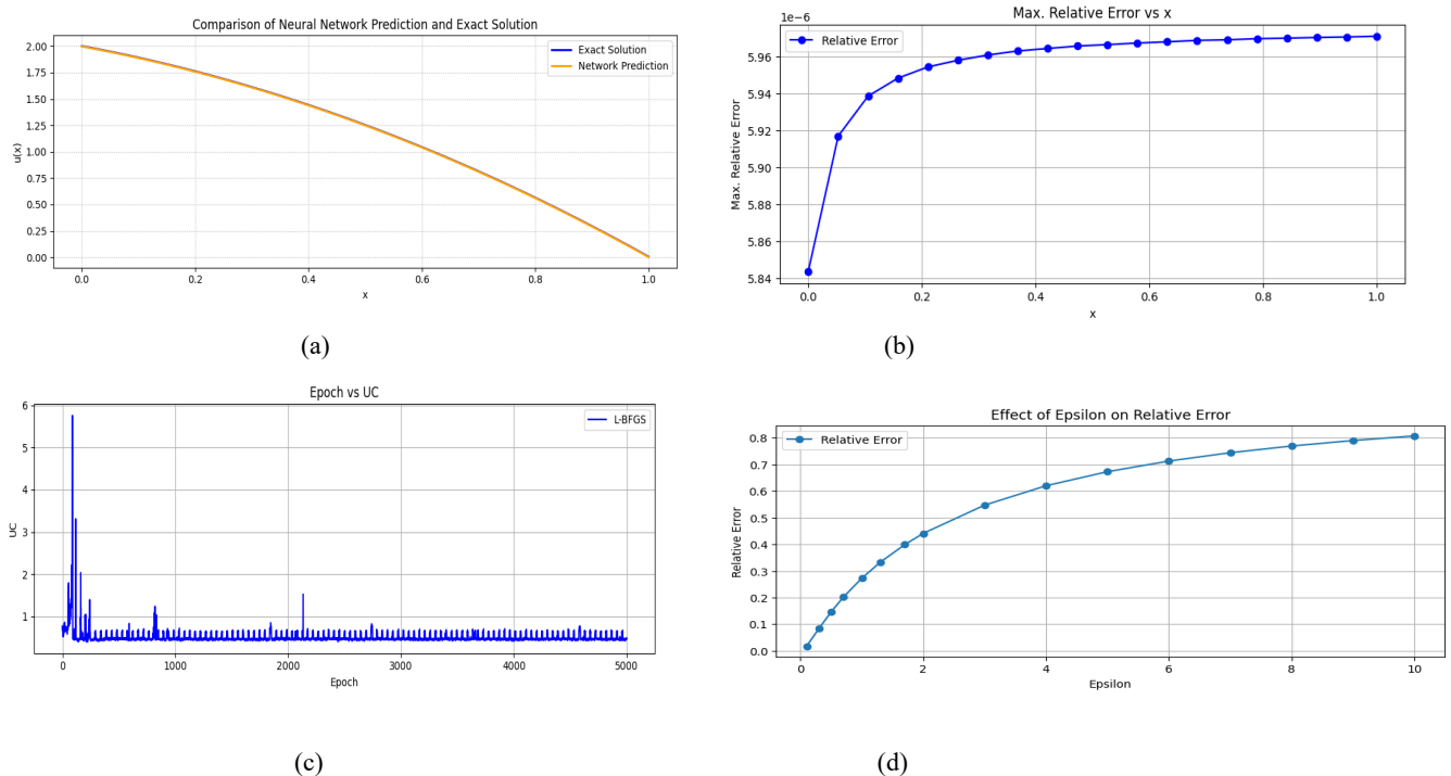
Figure 5. PINN-predicted and exact solutions for the chemical reactor problem: (a) solution profiles, (b) maximum relative error across spatial domain, (c) optimizer update cost versus training epochs, and (d) influence of parameter \epsilon on the relative error, illustrating model sensitivity.
