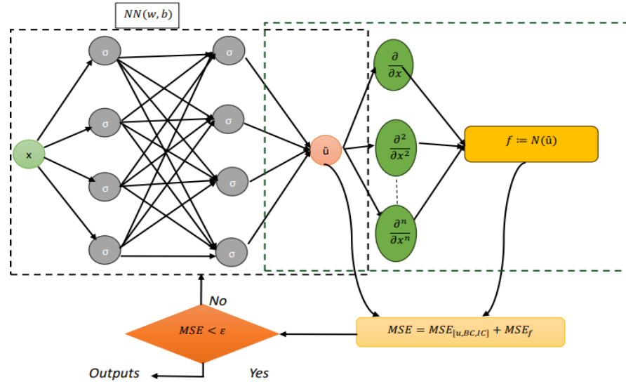
Figure 1. Methodology of the proposed cPINN, illustrating the network architecture, PDE residual computation at collocation points, and integration of causal training.
