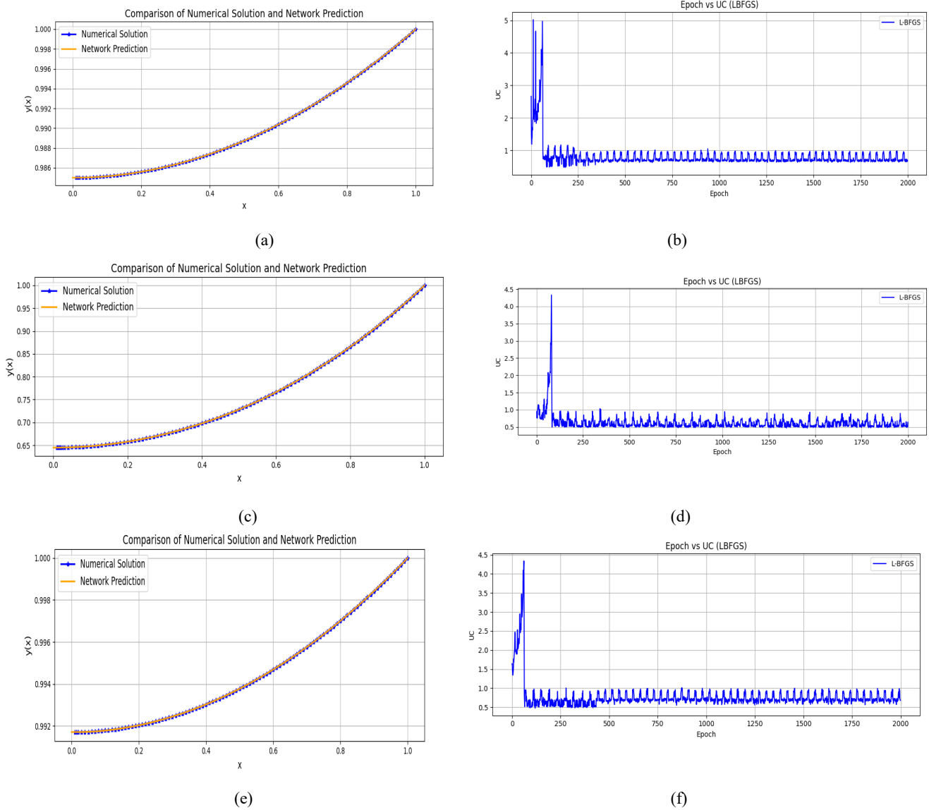
Figure 3. Comparison of PINN-predicted and exact solutions for the electroactive polymer film problem at different parameter settings: (a, c, e) show the solution profiles for cases (i) \alpha = 0.1, \mu = 0.1 , (ii) \alpha = 5, \mu = 1 , and (iii) \alpha = 0.1, \mu = 1 , respectively. Corresponding plots (b, d, f) display the optimizer update cost versus training epochs, illustrating convergence behavior across these cases.
